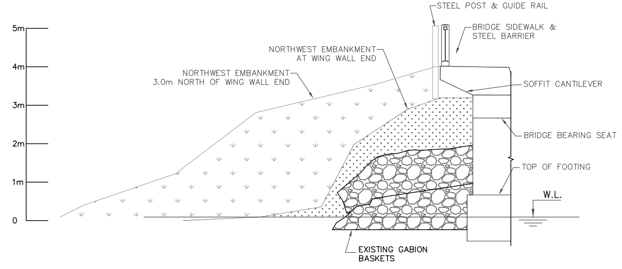
EXISTING NORTH ELEVATION 1:50
