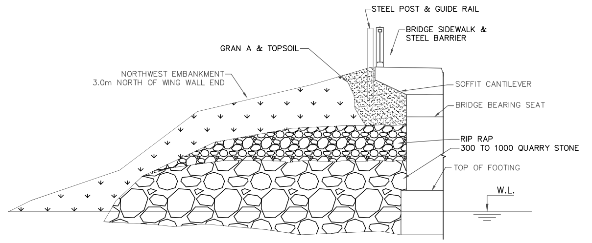
RECONSTRUCTED NORTHWEST EMBANKMENT FRONT ELEVATION 1:50
