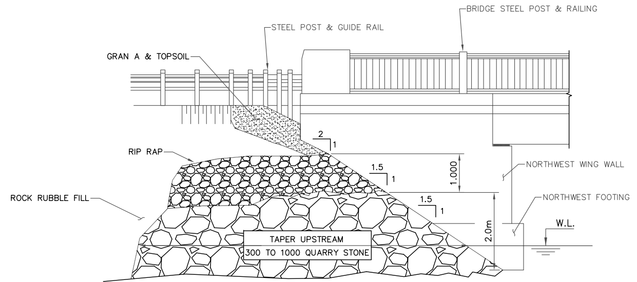
RECONSTRUCTED NORTHWEST EMBANKMENT WEST ELEVATION 1:50
