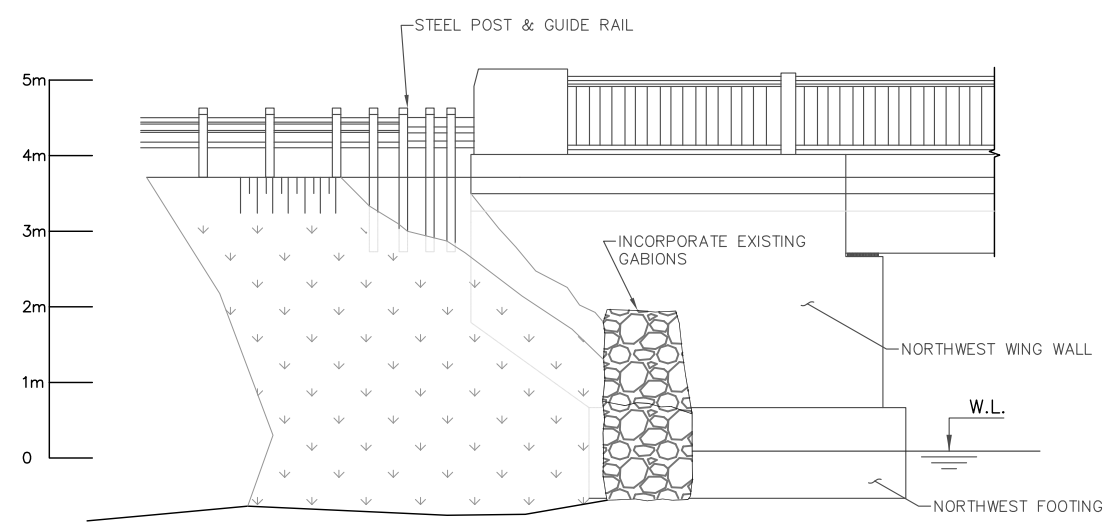
EXISTING WEST ELEVATION 1:50
